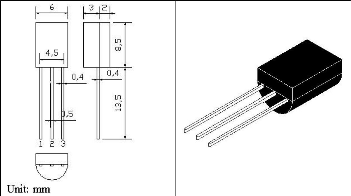
TO-92MOD
