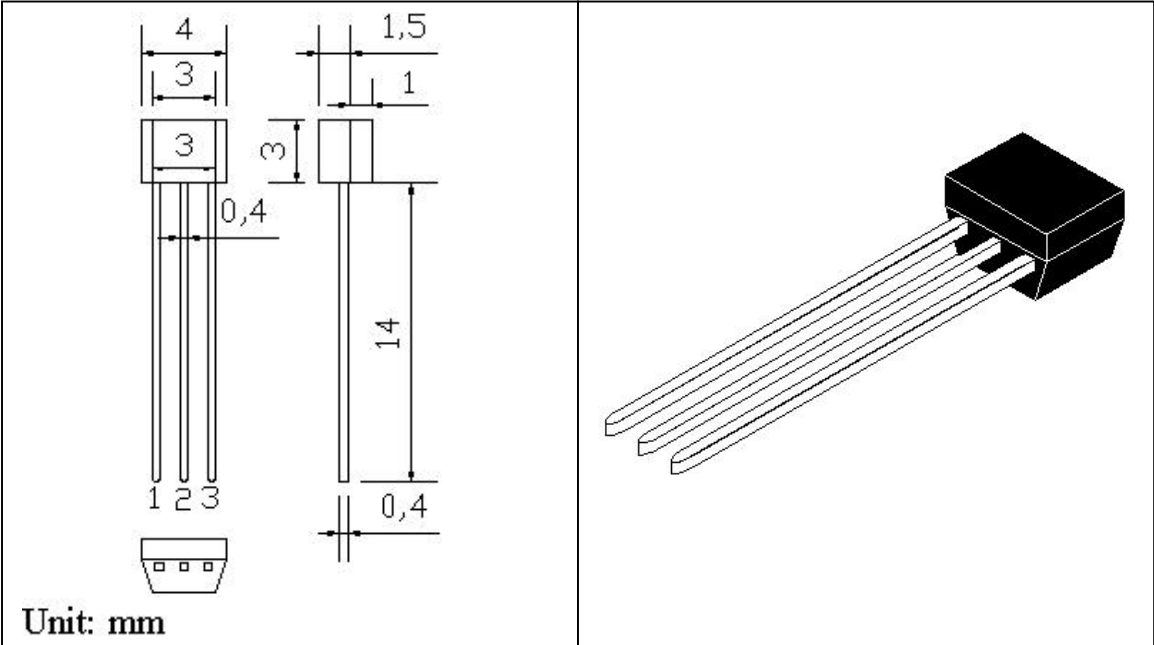
TO-92S
